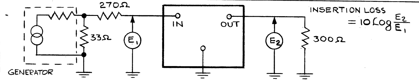
TEST SCHEMATIC
