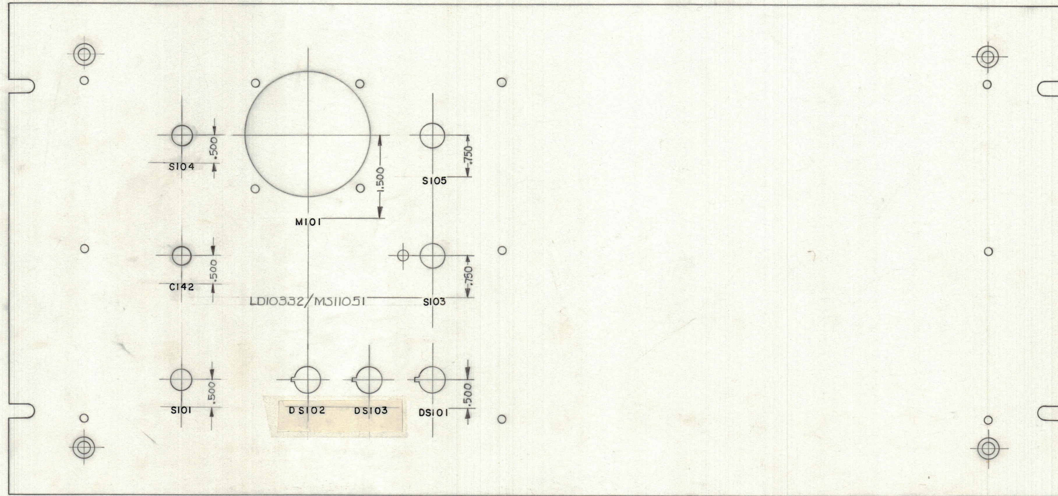
REAR VIEW OF FRONT PANEL
