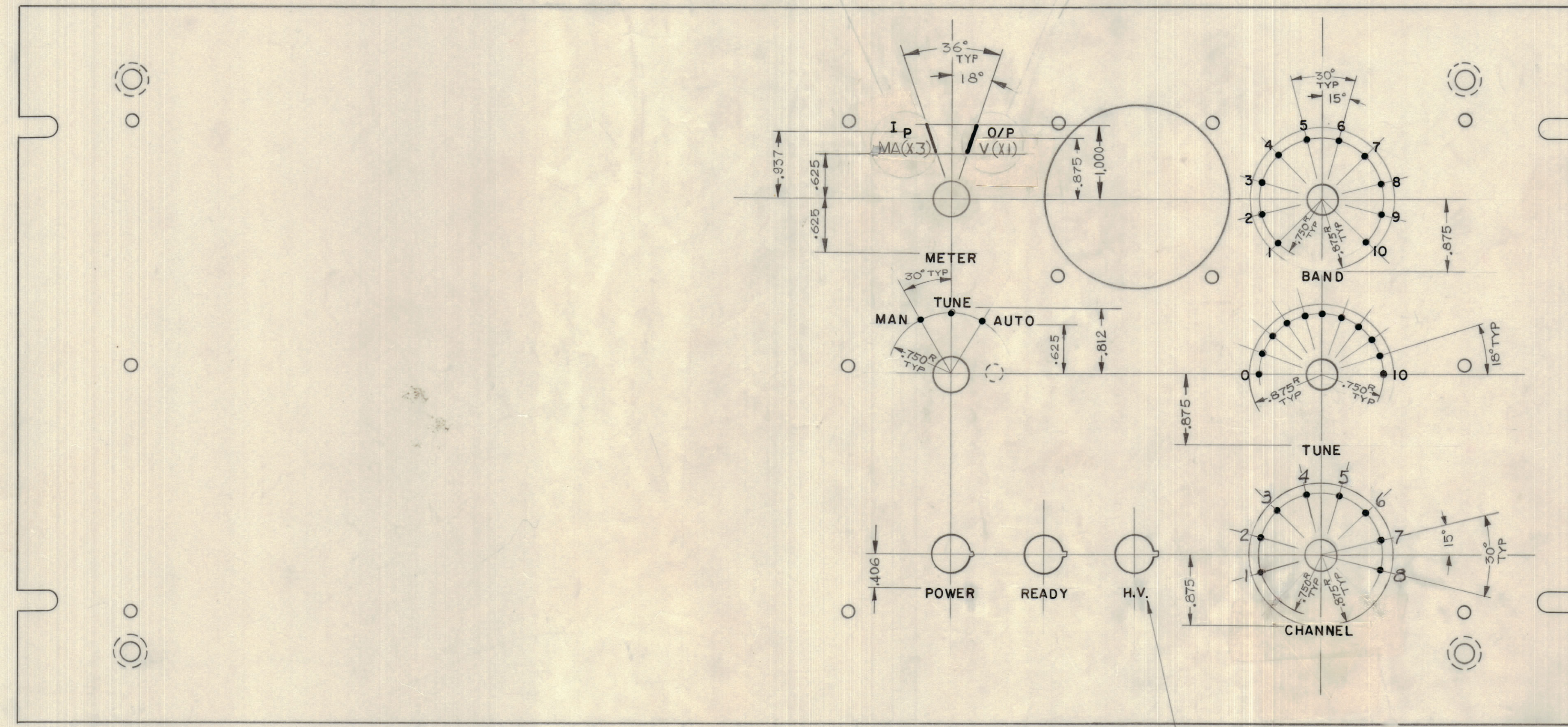
FRONT OF PANEL
