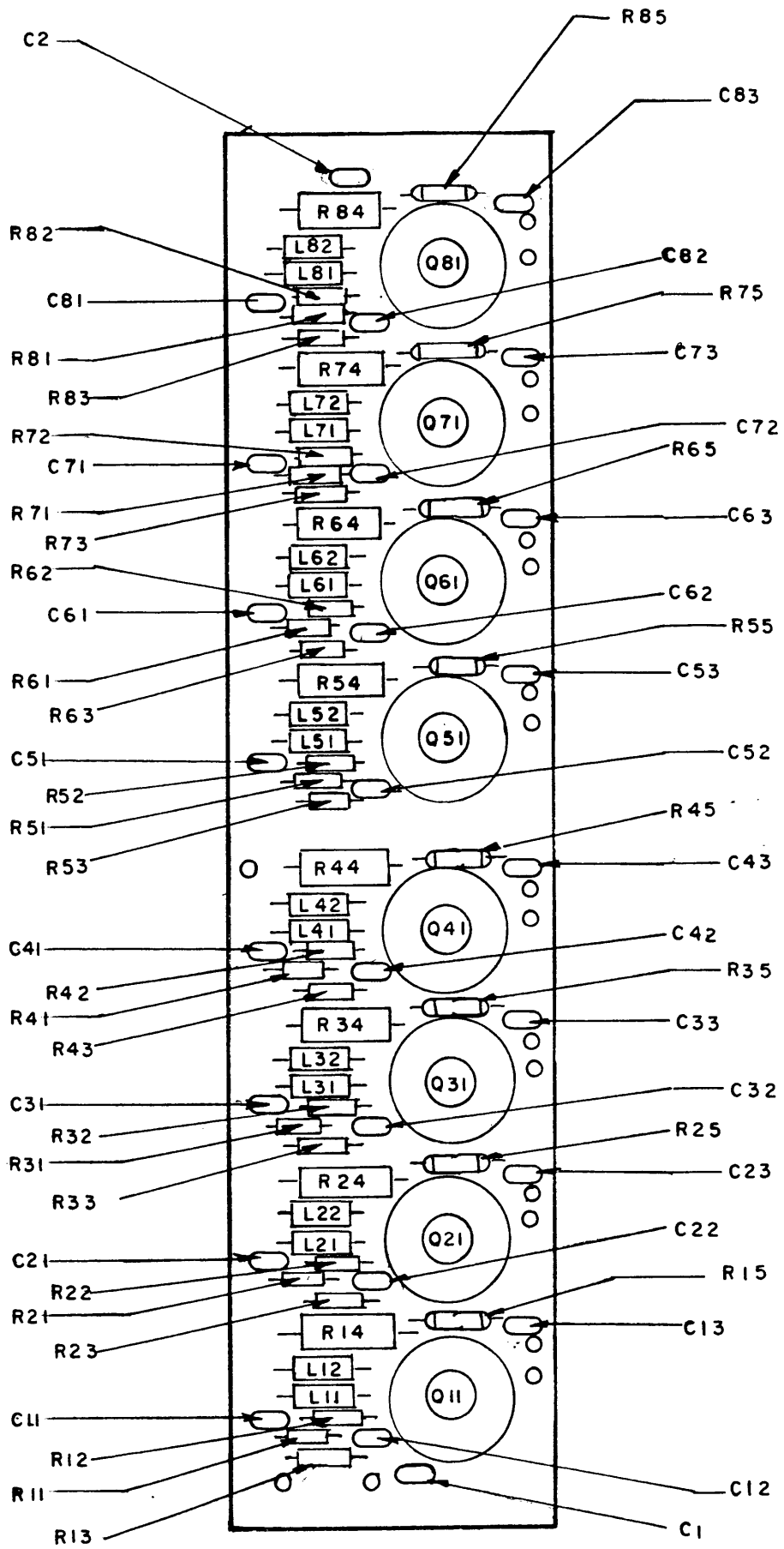
Figure 5-6 8 Output Assembly 1A4
