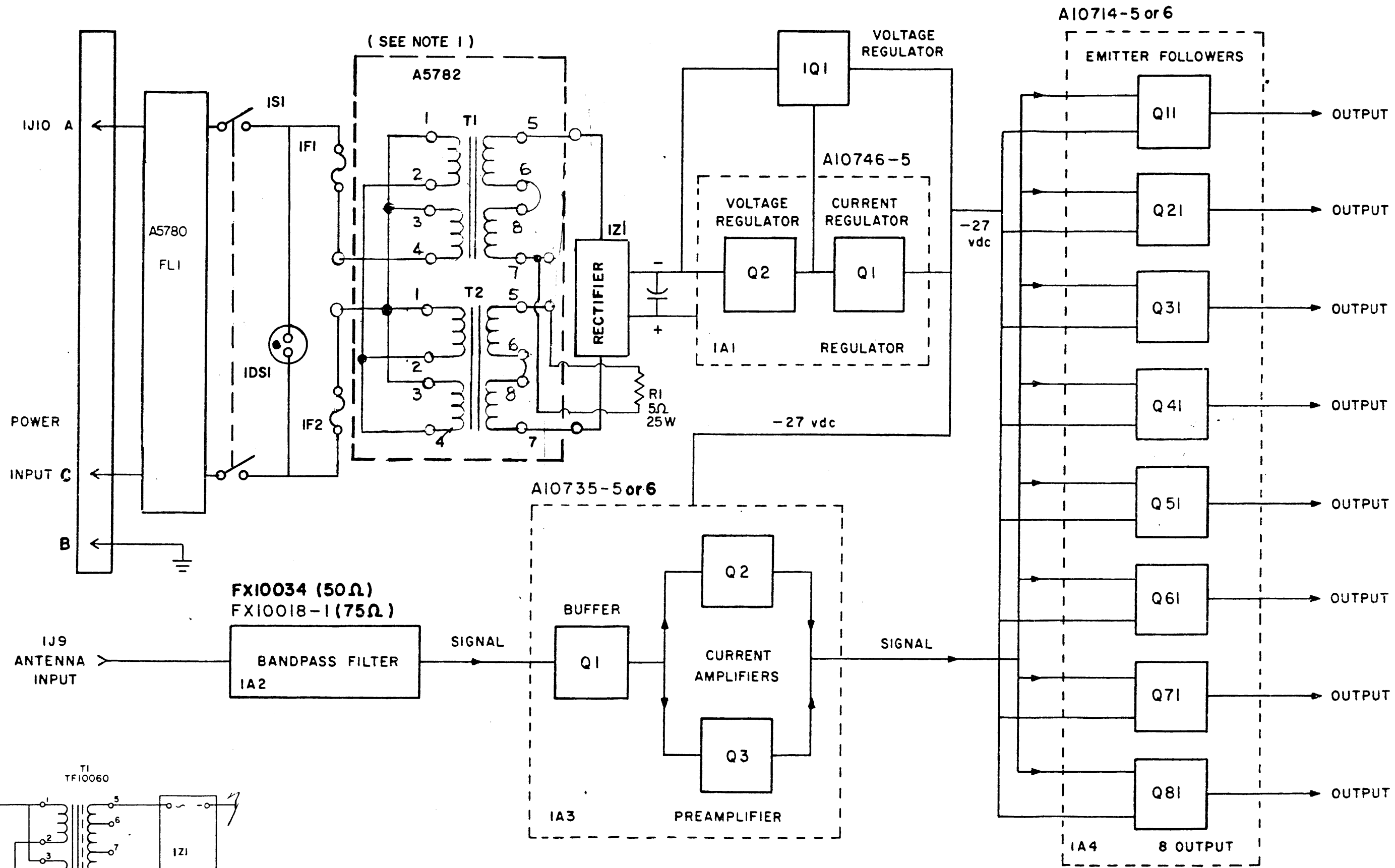
Figure 4-1 System Block Diagram, AMC-8A
