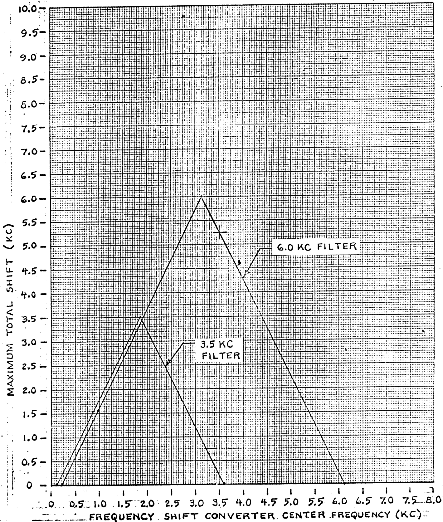
FIGURE 3-2. FSK CONVERTER CENTER FREQUENCY VS. DDR-7 B SHIFT CAPABILITIES
