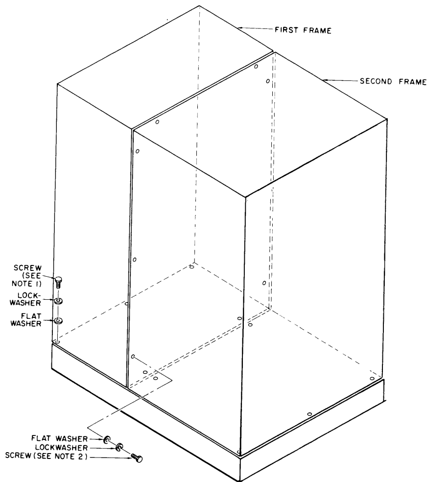
Figure 2-6. First and Second Frames, Installation Diagram.
