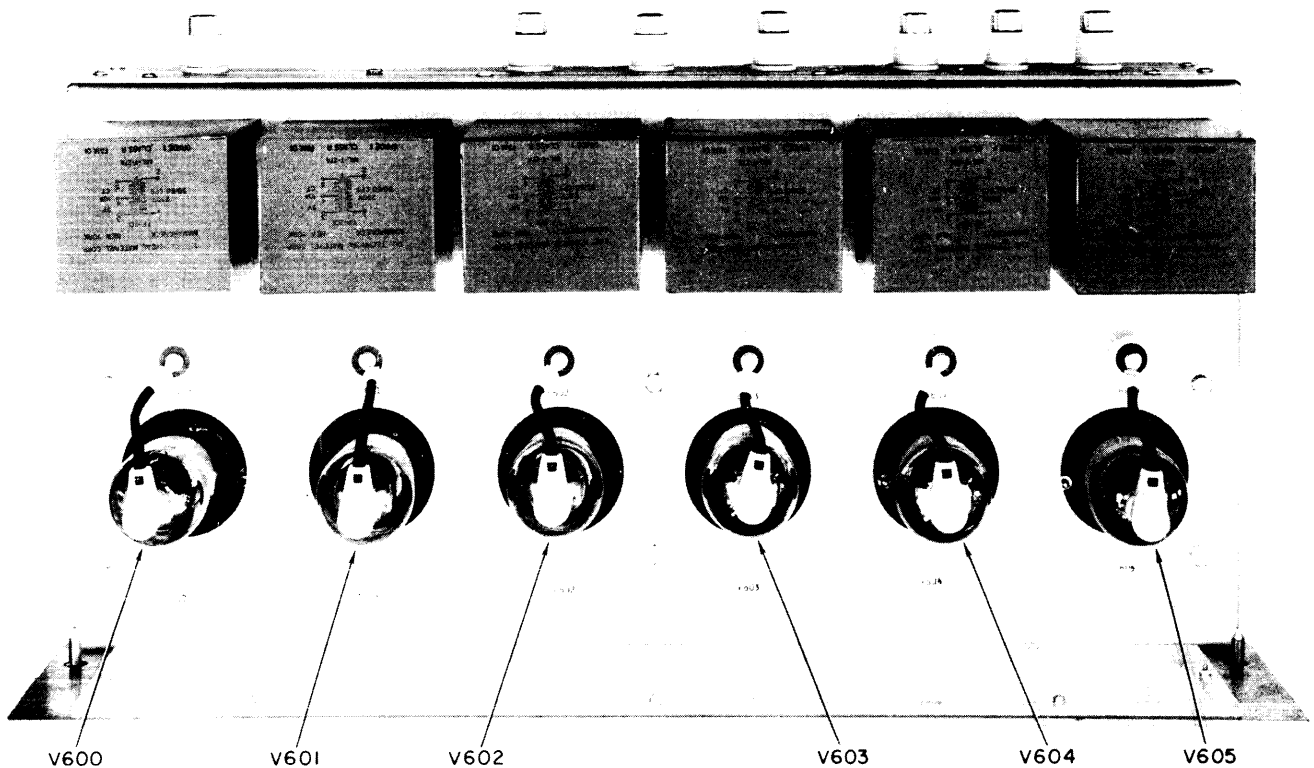
Figure 2-14. High Voltage Rectifier Drawer 600, Top View.
