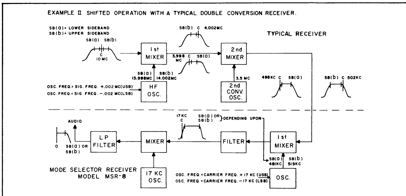
Figure 2-2. Block Diagram (Example II) MSR-8/Typical Receiver
