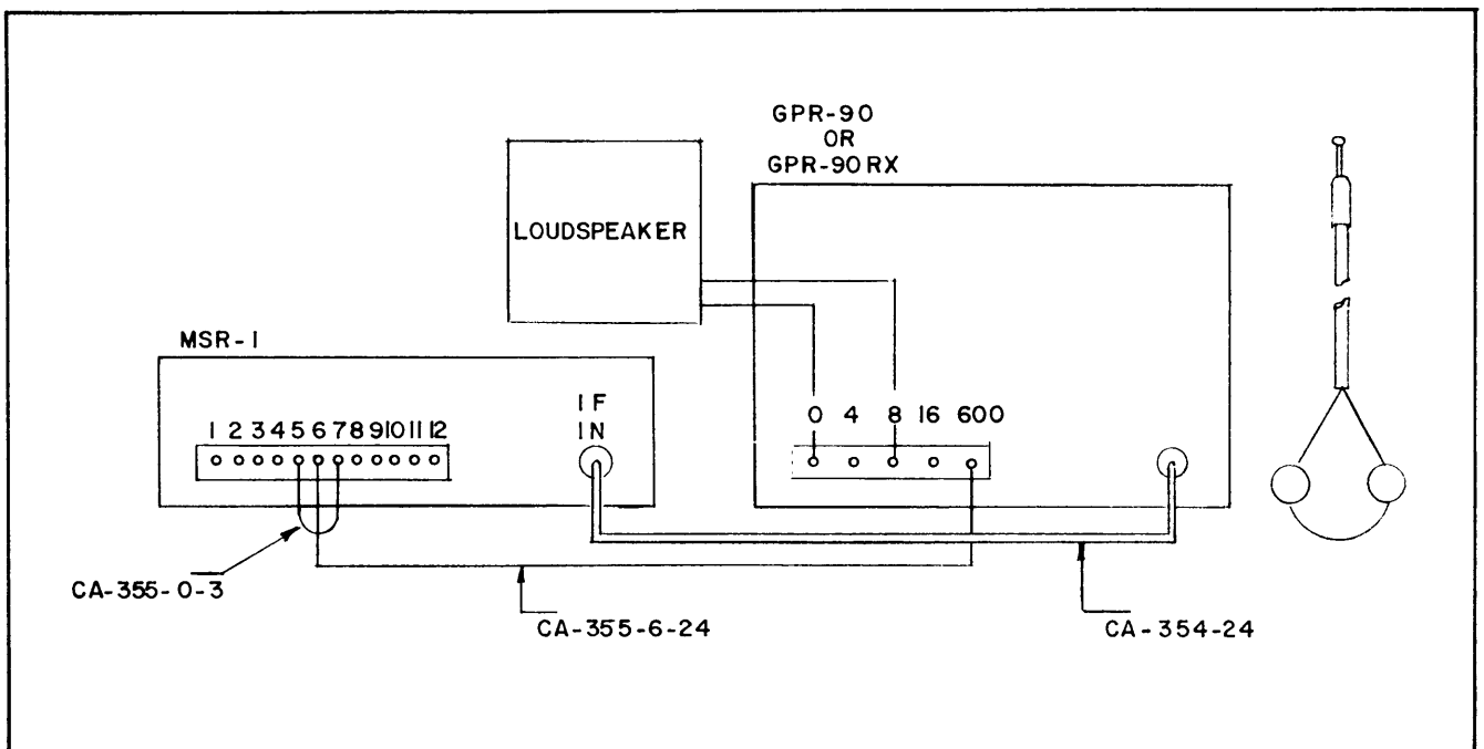
Figure 3-1. Cabling Connections Models MSR-4/GPR-90 for Single Loudspeaker Operation
