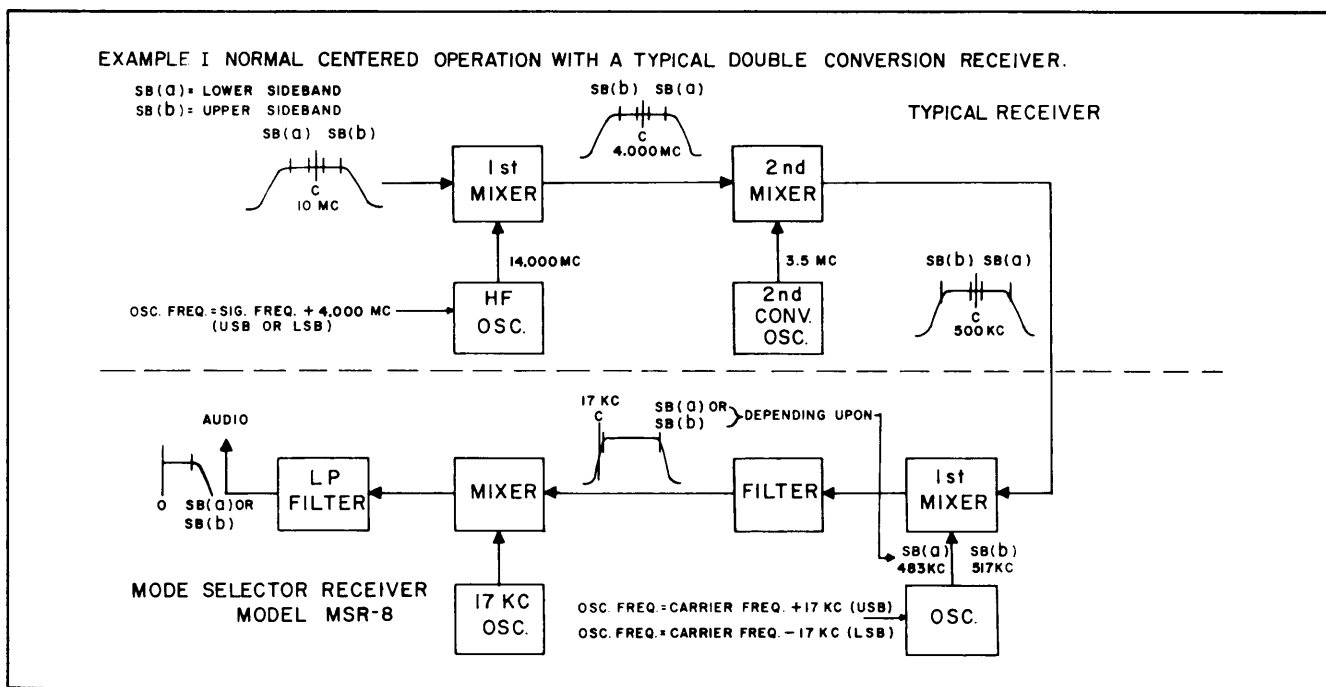
Figure 2-1. Block Diagram (Example I) MSR-8/Typical Receiver
