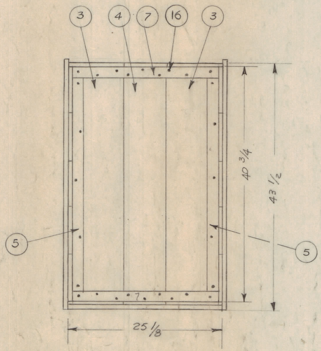
END VIEW
