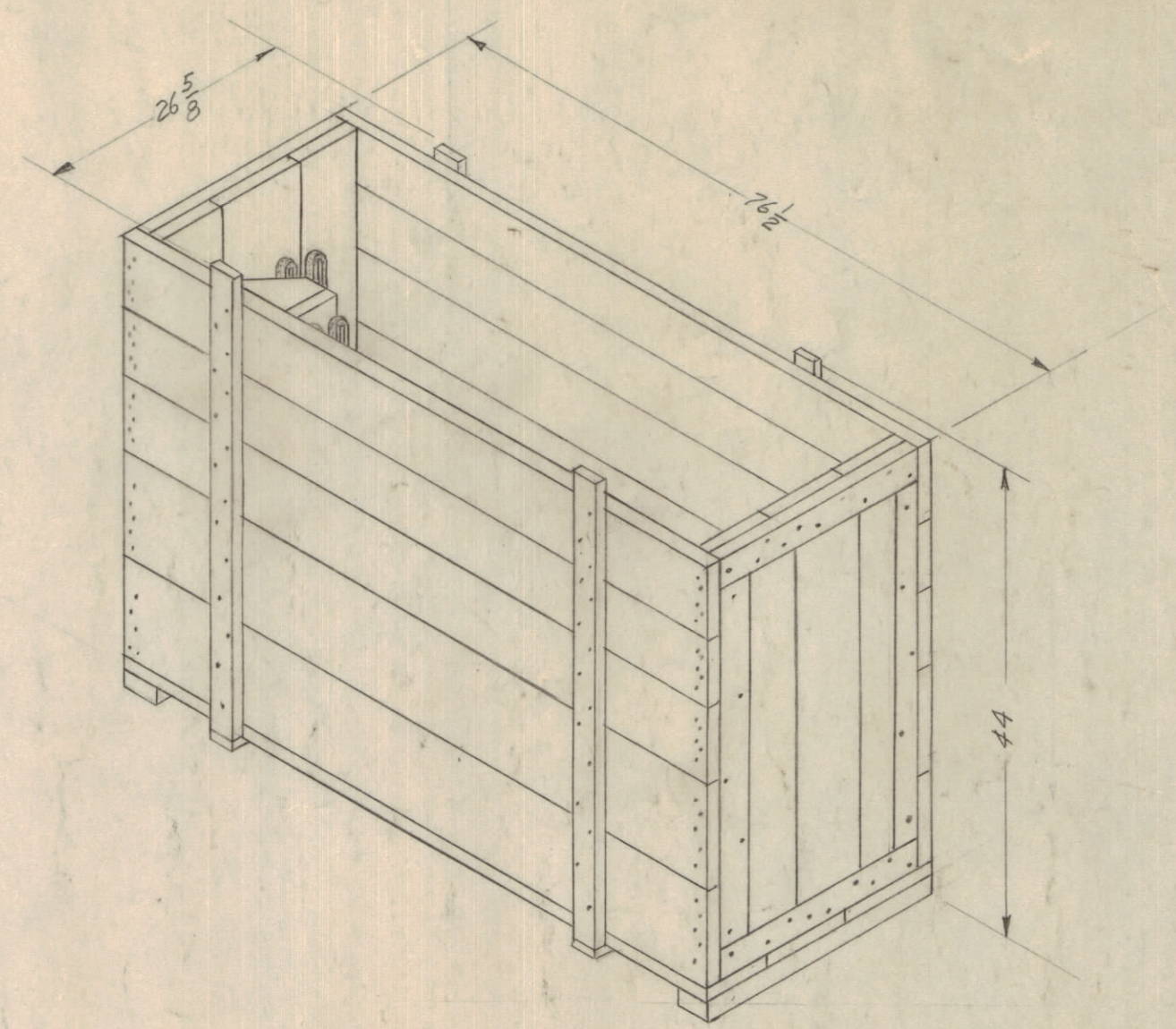
ISOMETRIC OF BXW-103 SHOWN W/COVER REMOVED
