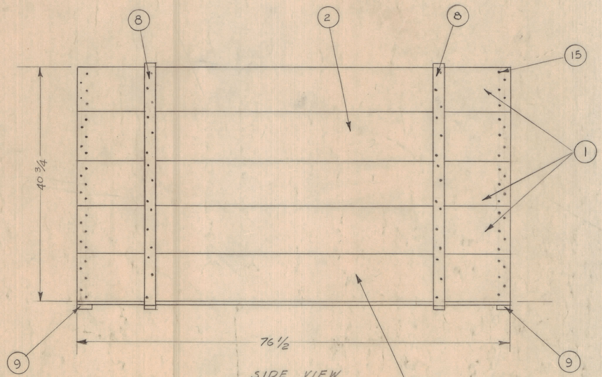
SIDE VIEW
