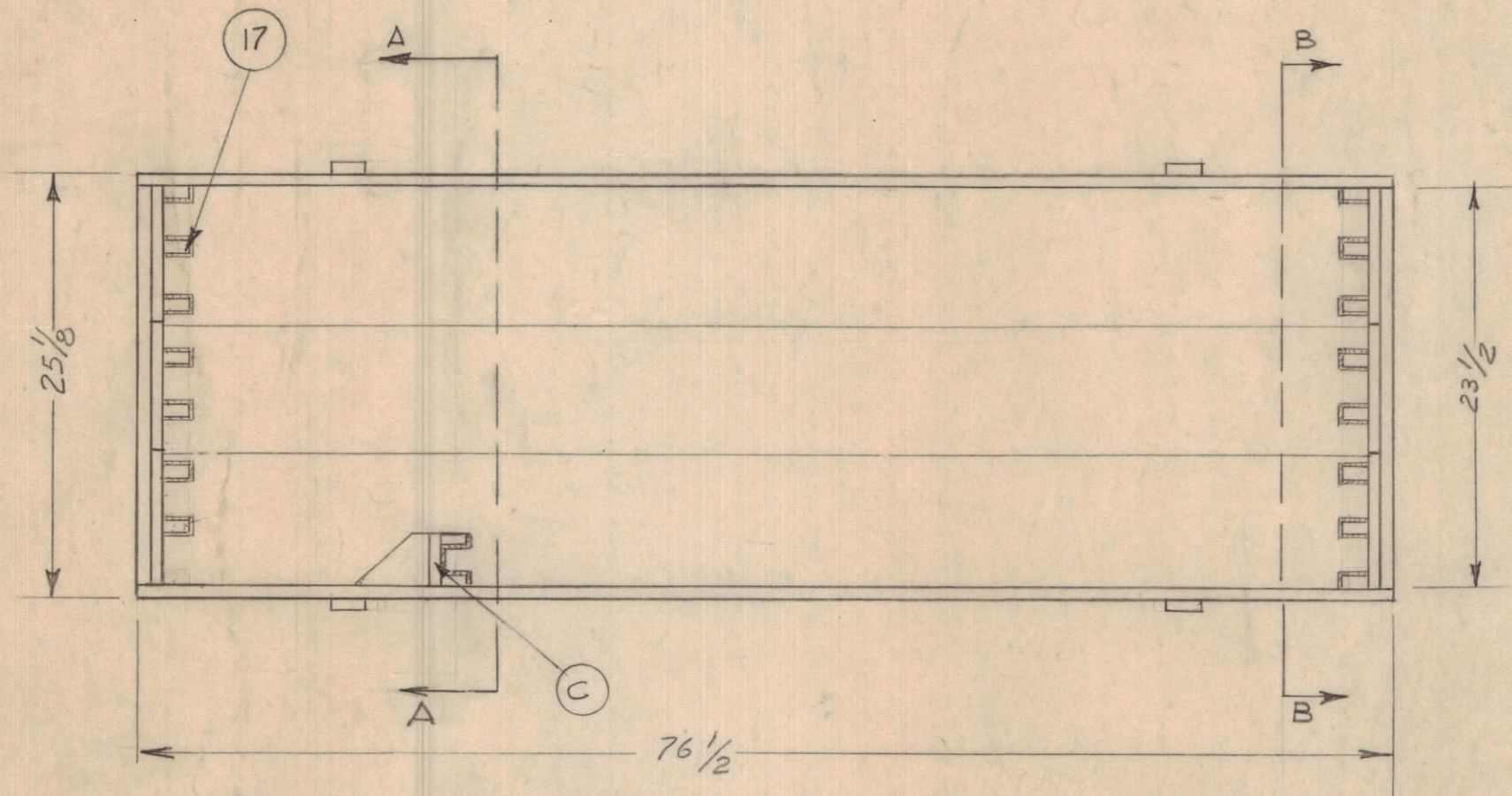
TOPE VIEW W/COVER REMOVED
