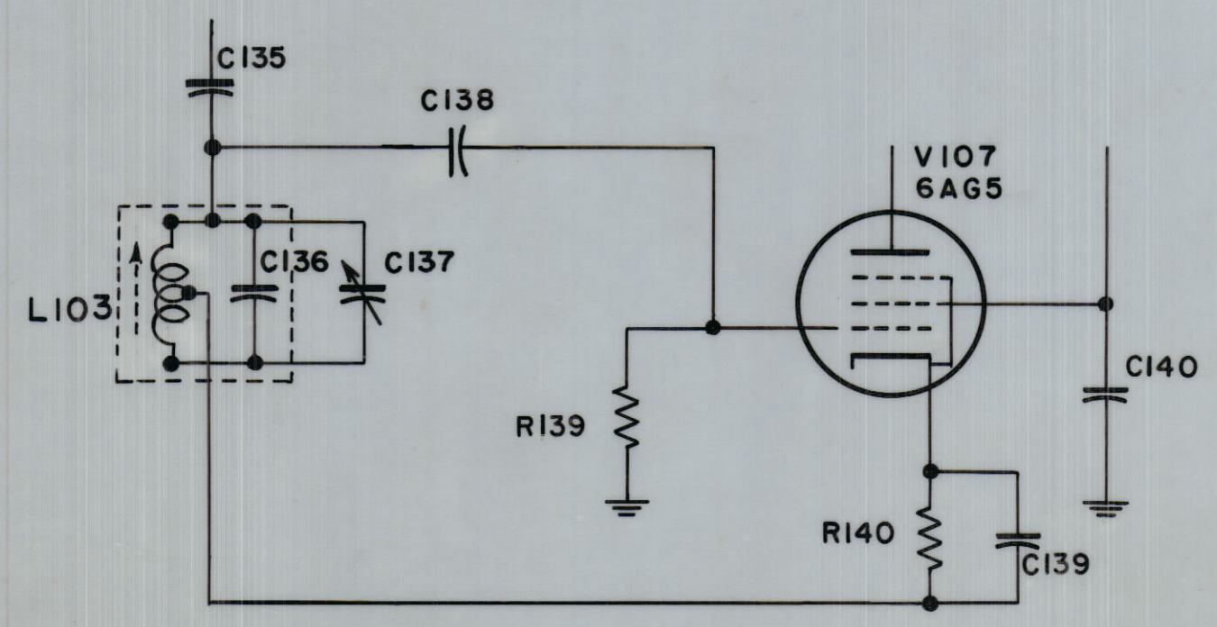
S103 IN POSITION 3 (BFO)
