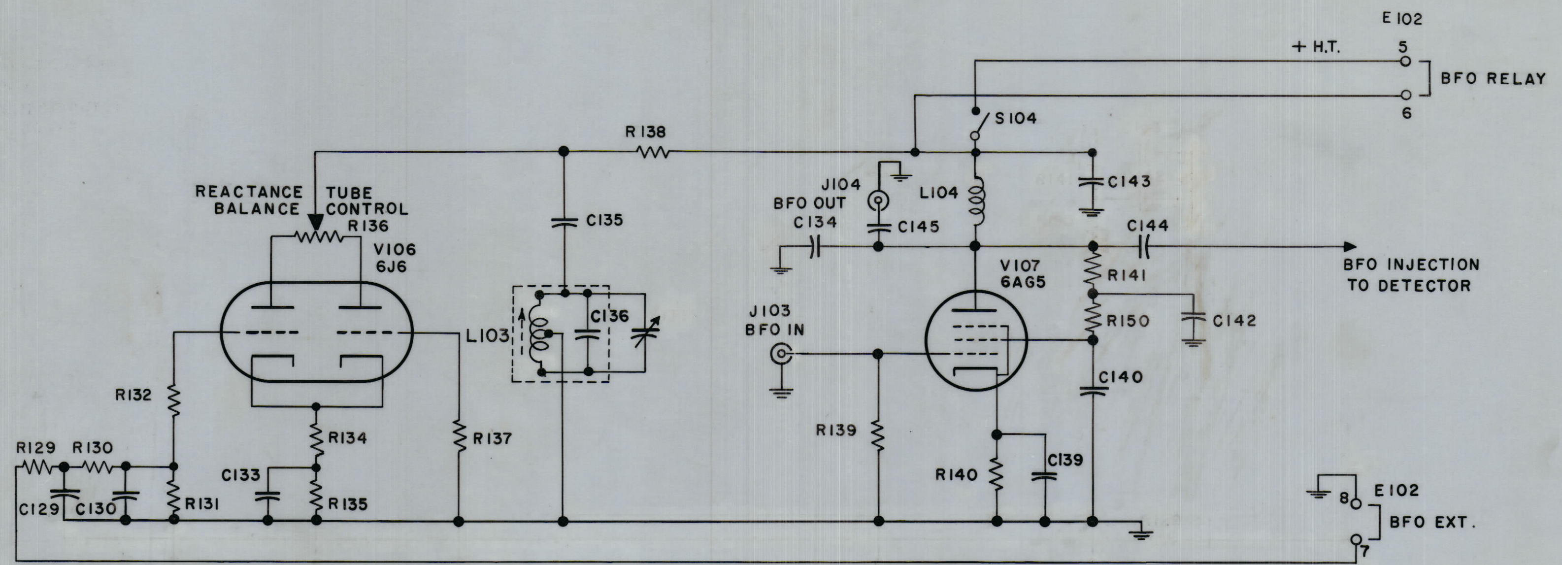
SIMPLIFIED BFO & BFO REACTANCE CIRCUIT S103 IN POSITION 1. (EXT-SLAVE)
