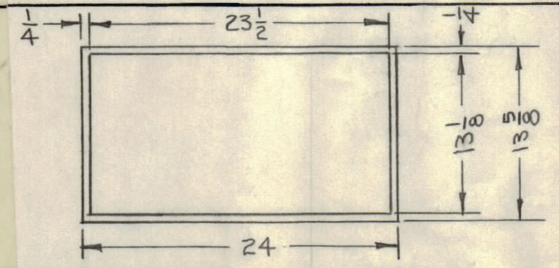
LAMINATING DETAIL MATERIAL: VINYL PLASTIC .015
