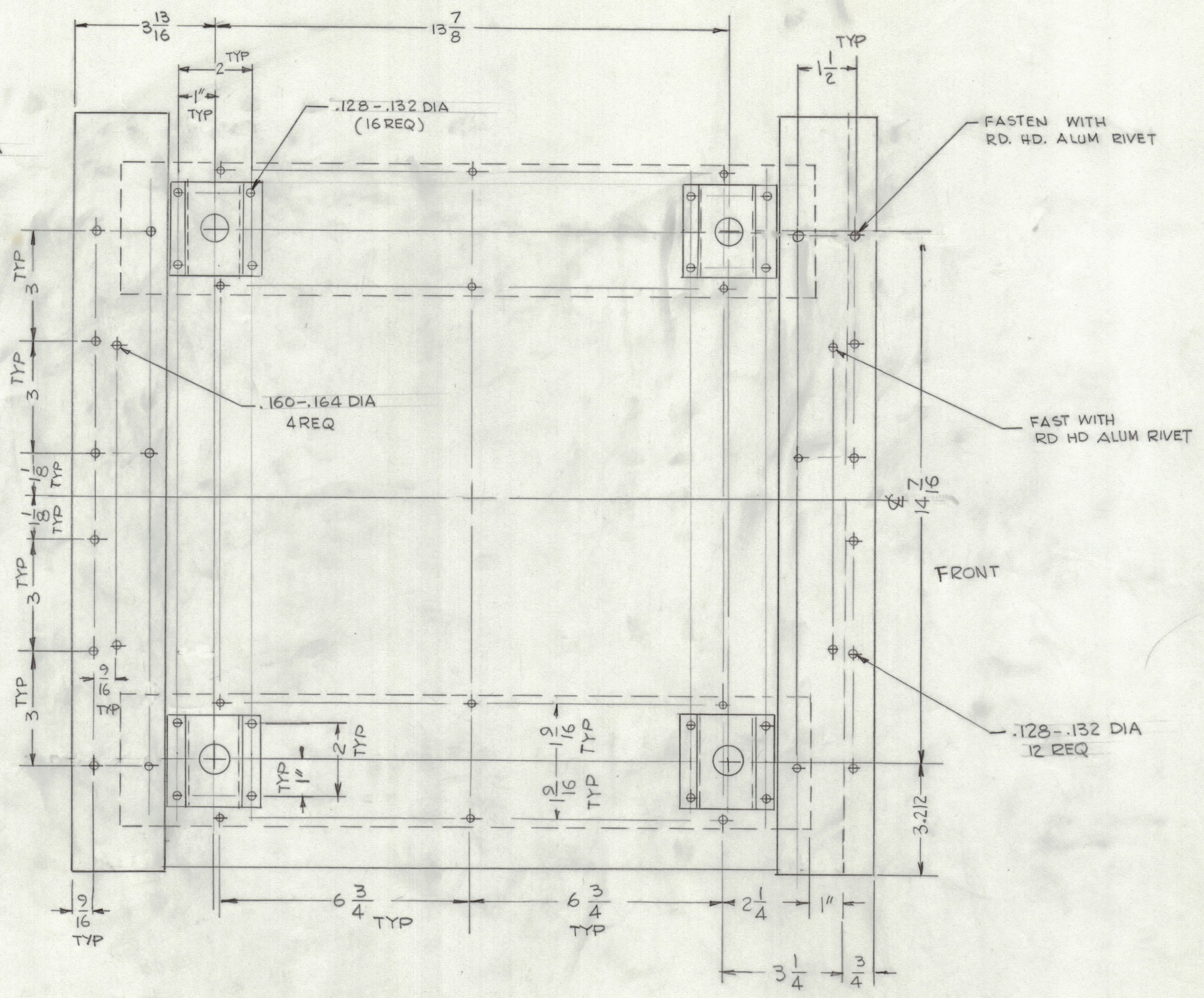
— BOTTOM VIEW —
