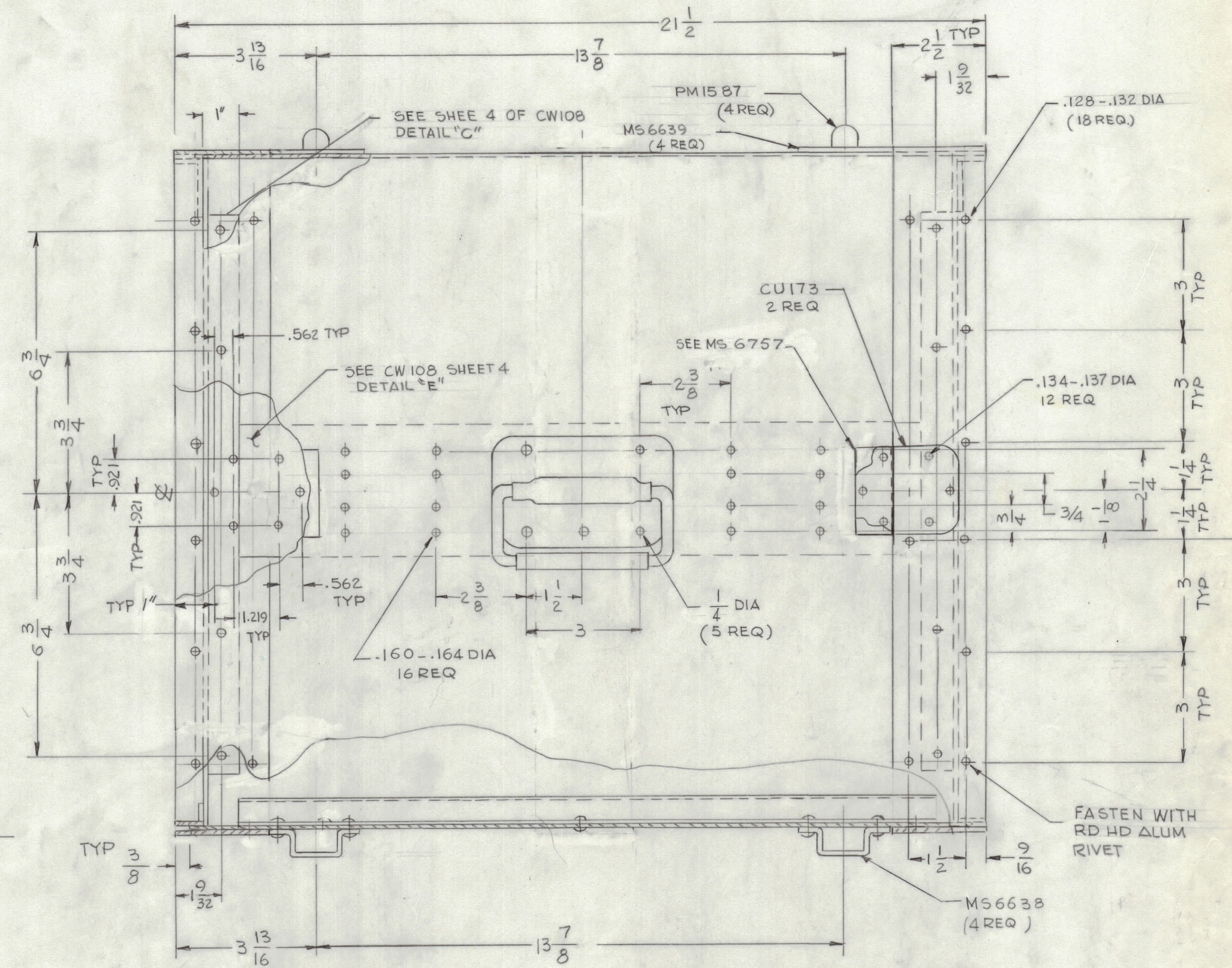
RIGHT SIDE VIEW (COVER REMOVED)
