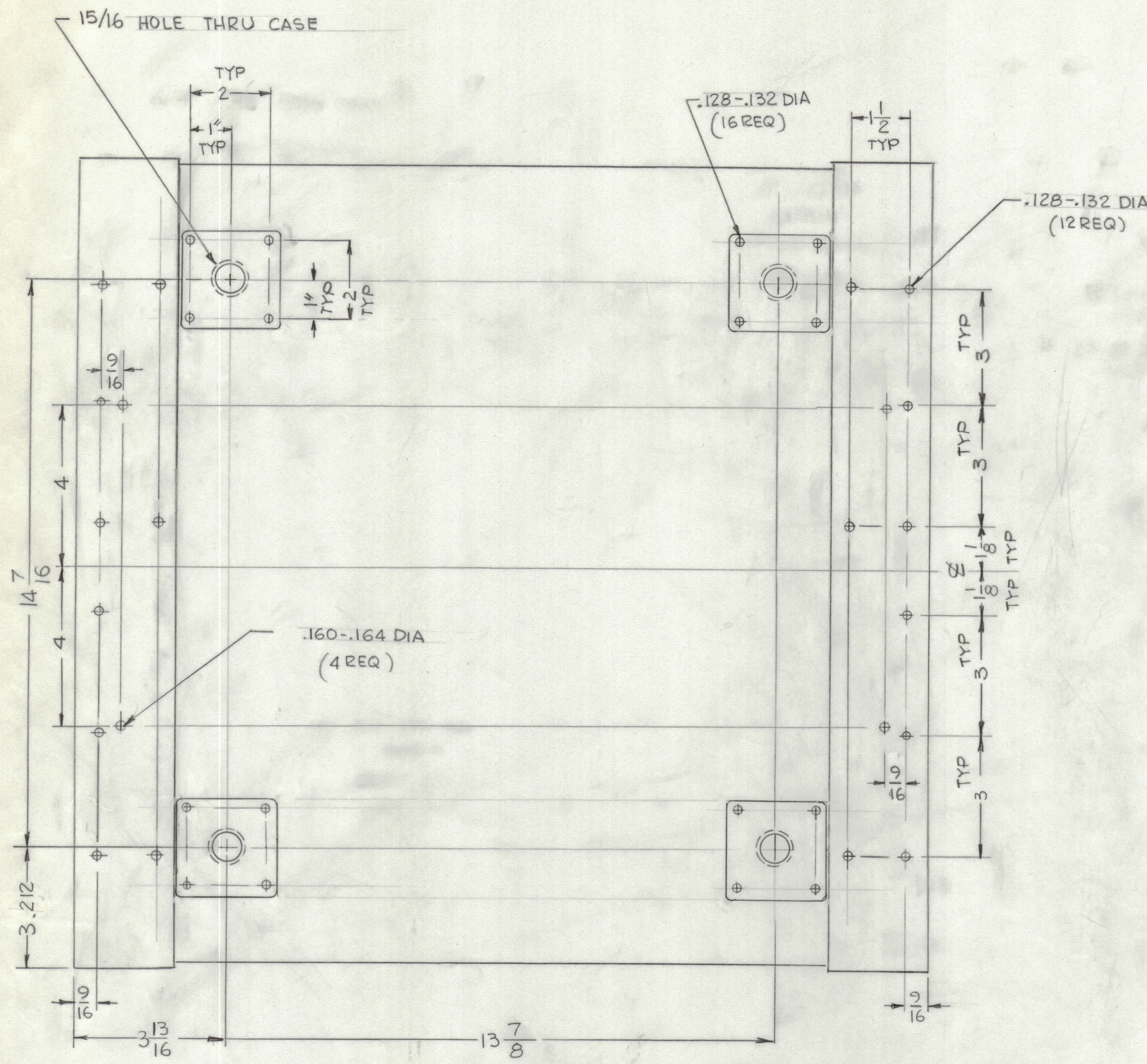
— TOP VIEW —
