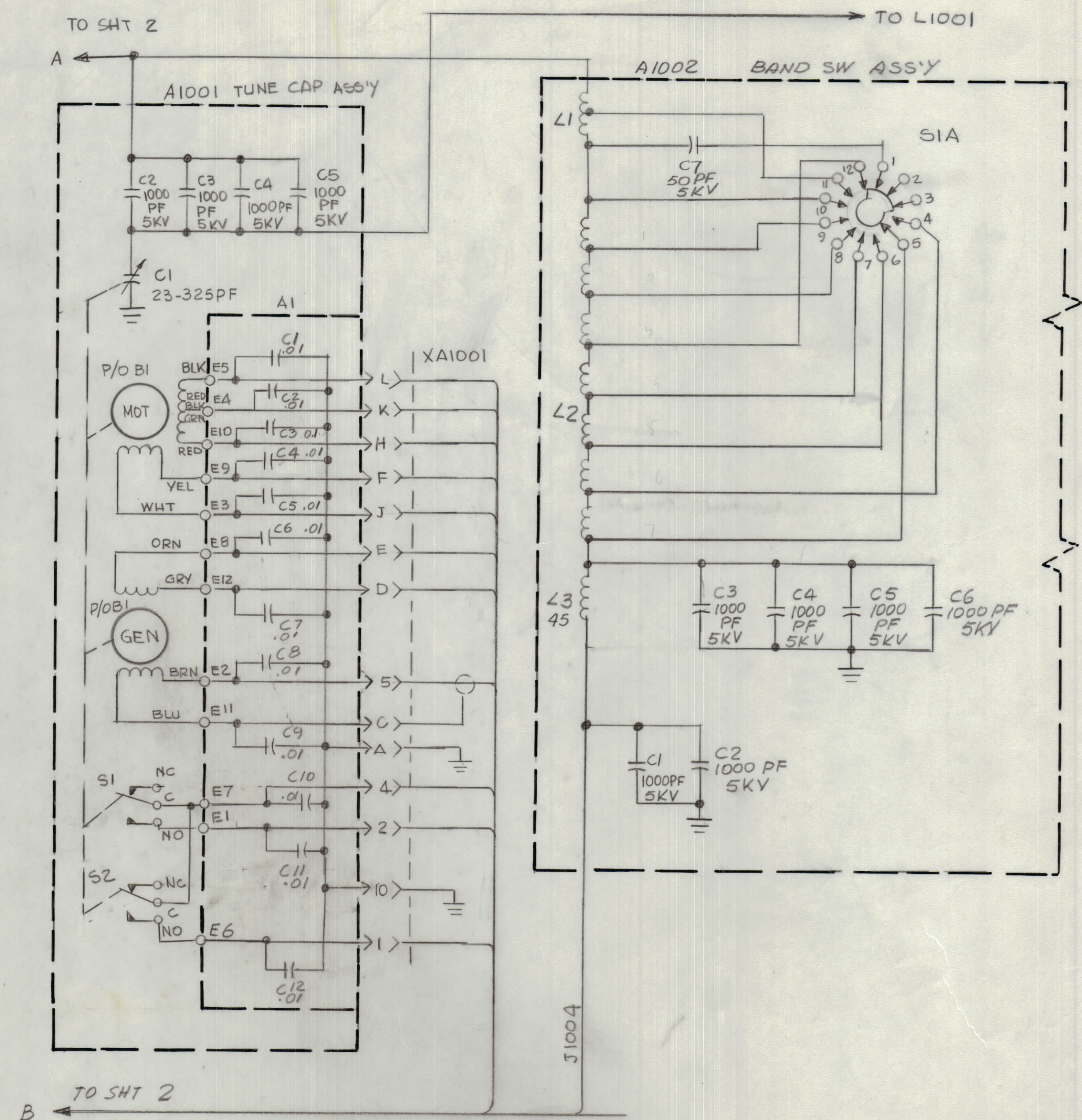
SCHEMATIC BEFORE MODIFICATION
