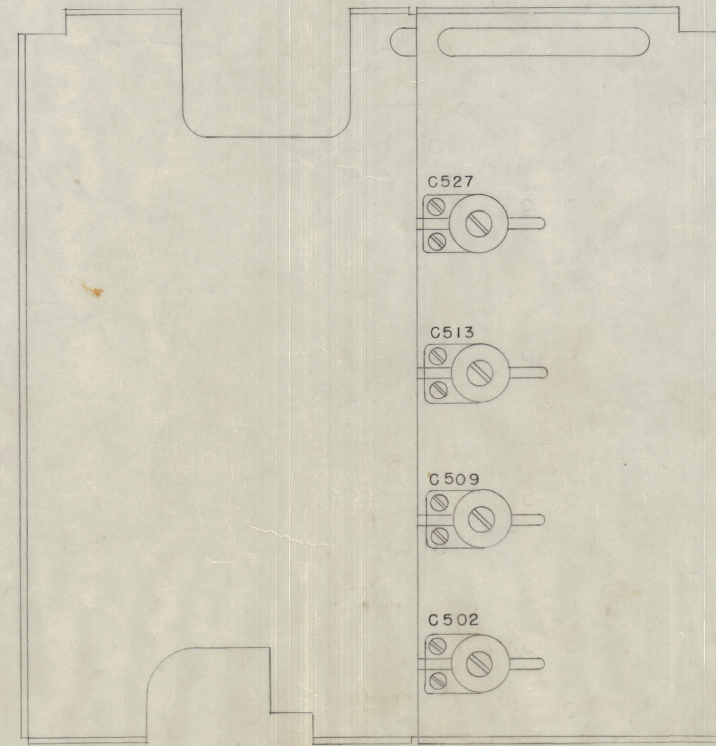
CHASSIS BOTTOM
