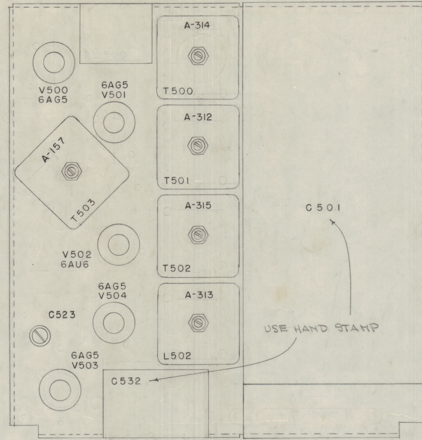
CHASSIS TOP
