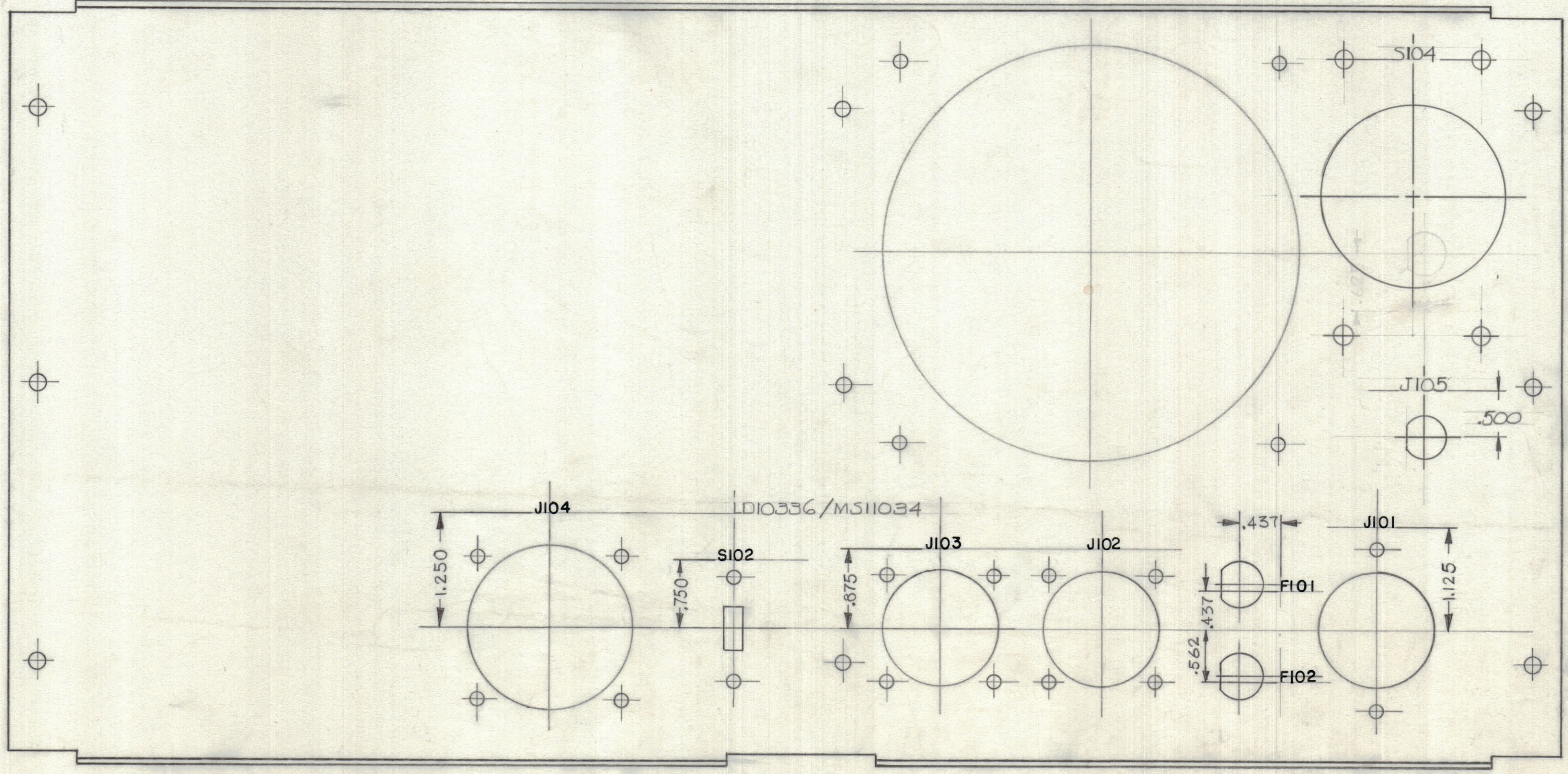
REAR VIEW OF REAR PANEL
