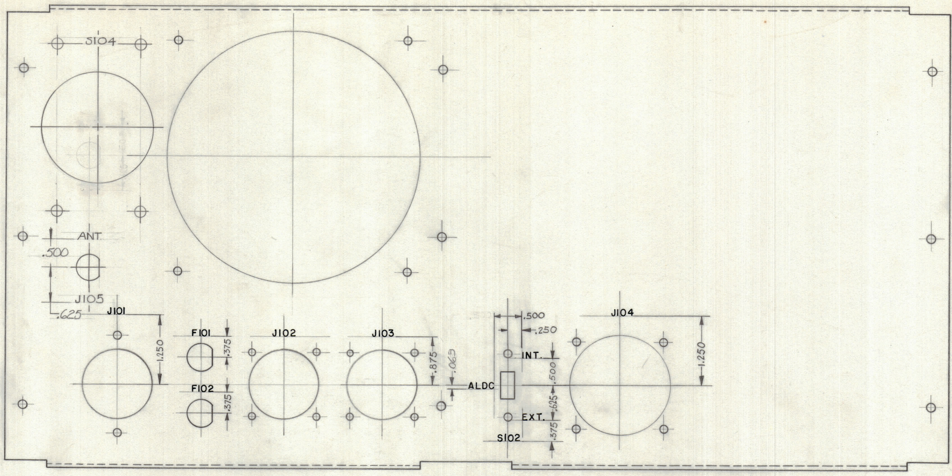
FRONT VIEW OF REAR PANEL
