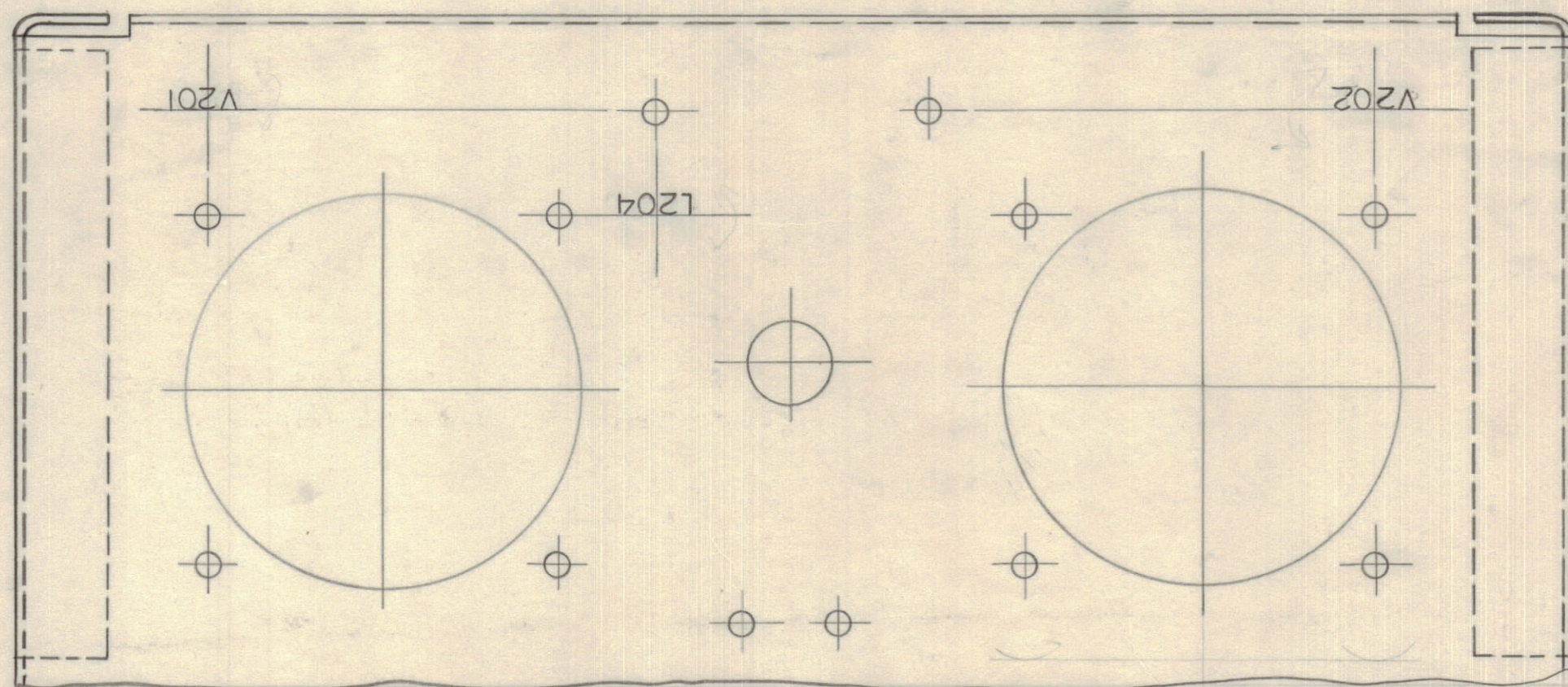
TOP SIDE VIEW OF REAR PART CHASSIS
