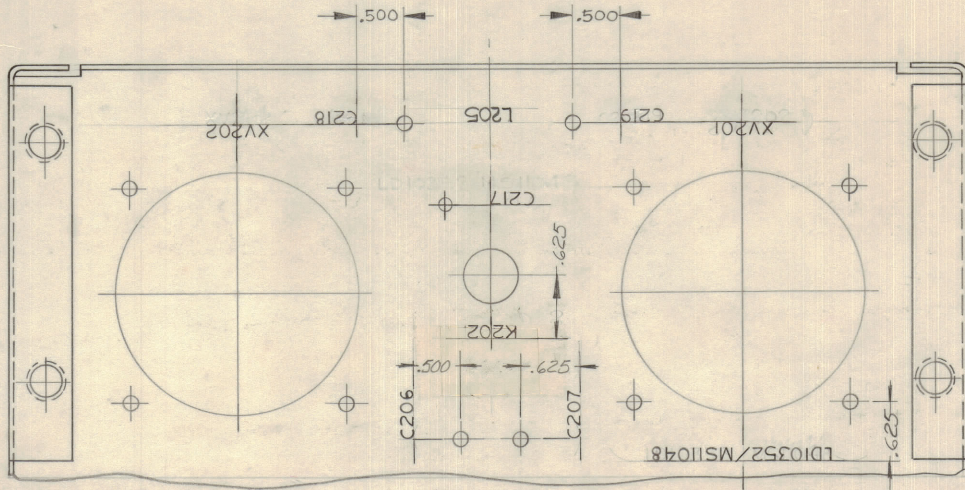
UNDER SIDE VIEW OF REAR PART CHASSIS
