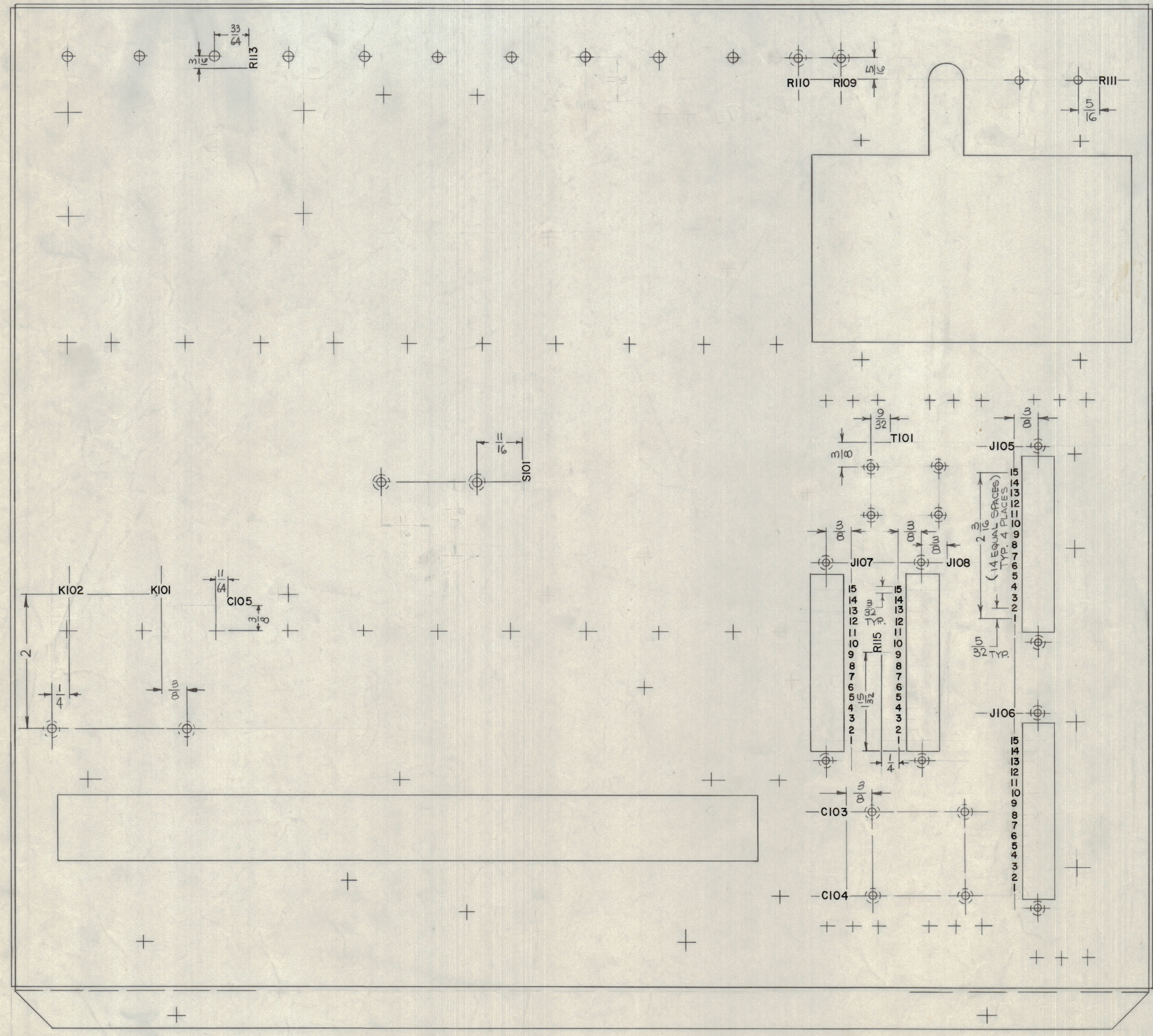
BOTTOM VIEW
