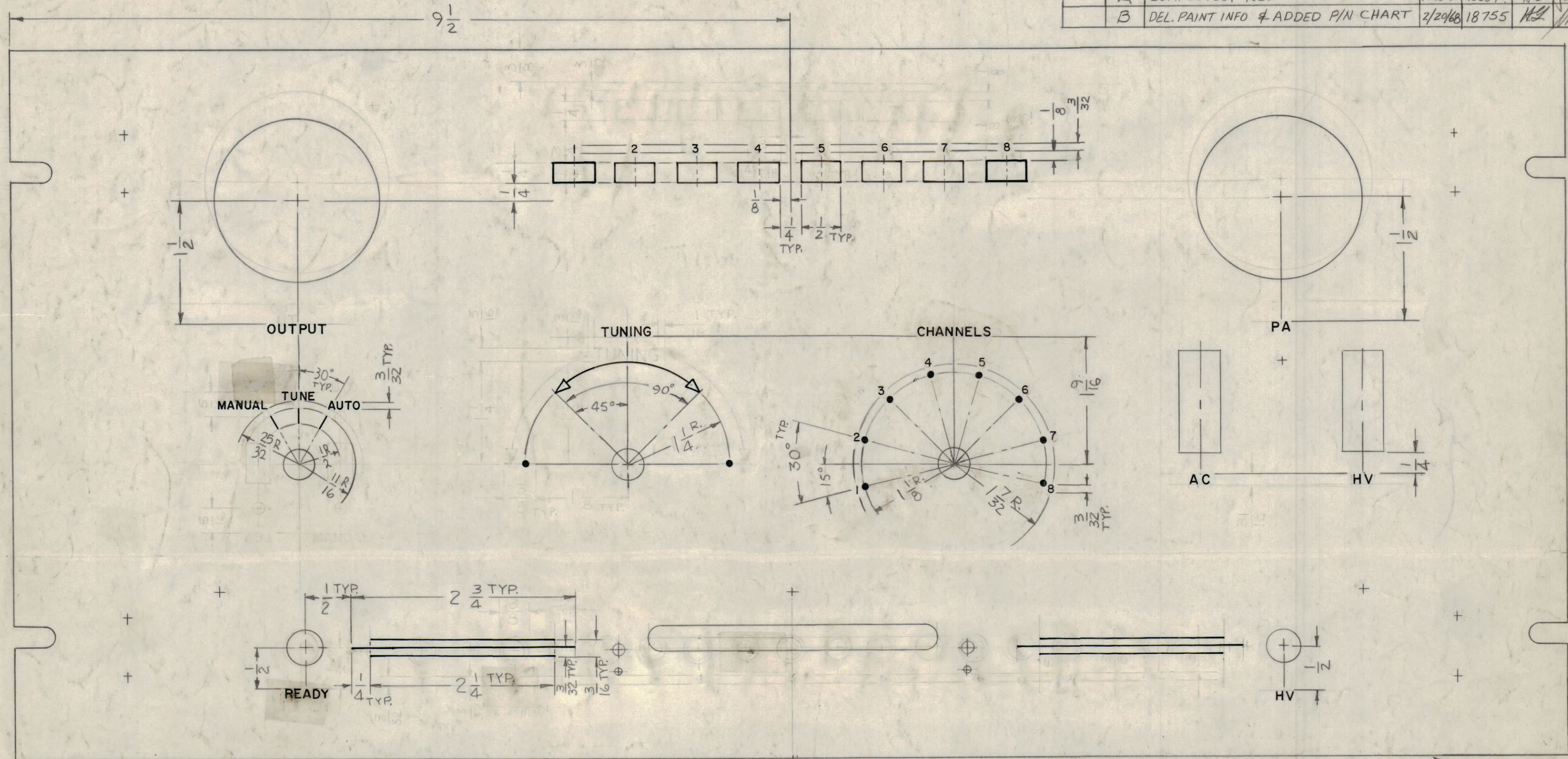
FRONT VIEW
