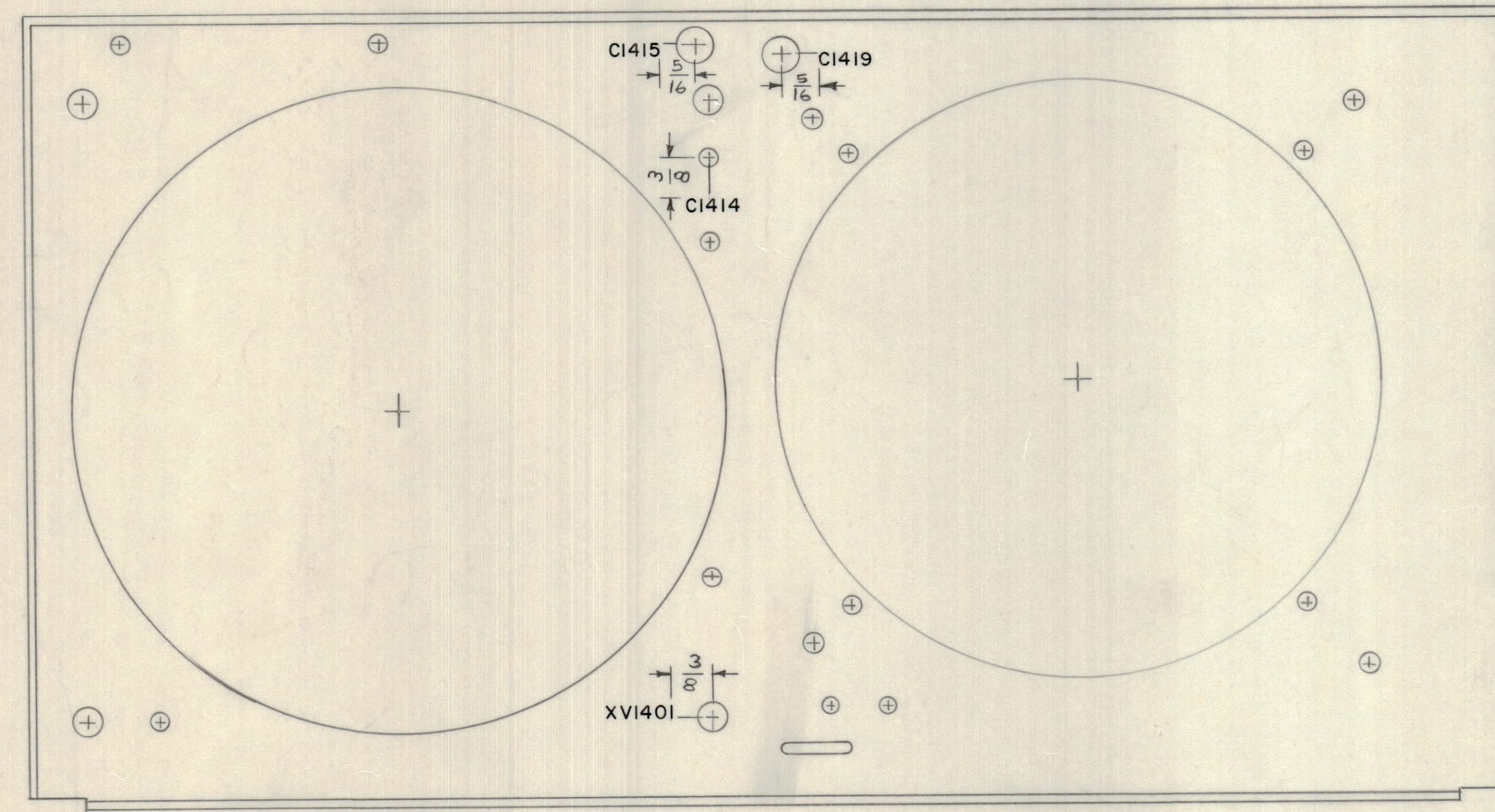
INSIDE VIEW
