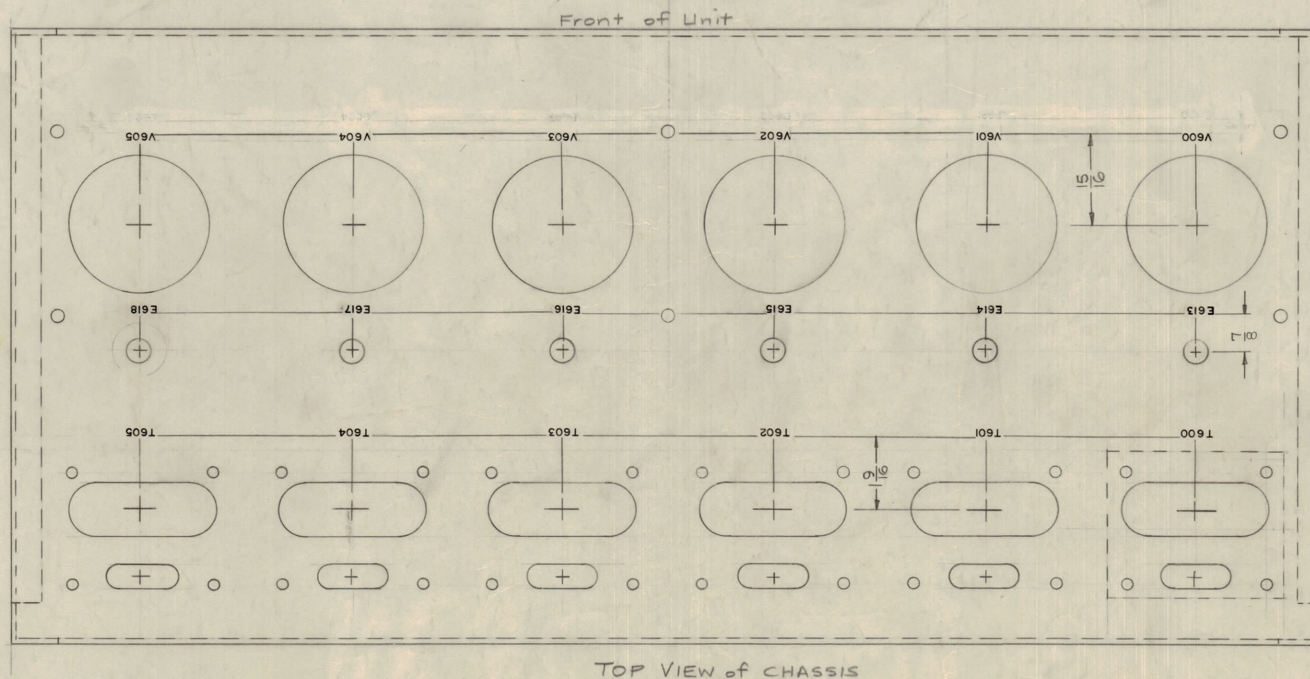
TOP VIEW of CHASSIS
