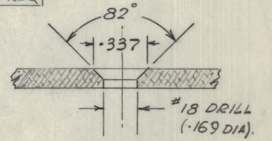
DETAIL J FOR #8-32 FHS.
