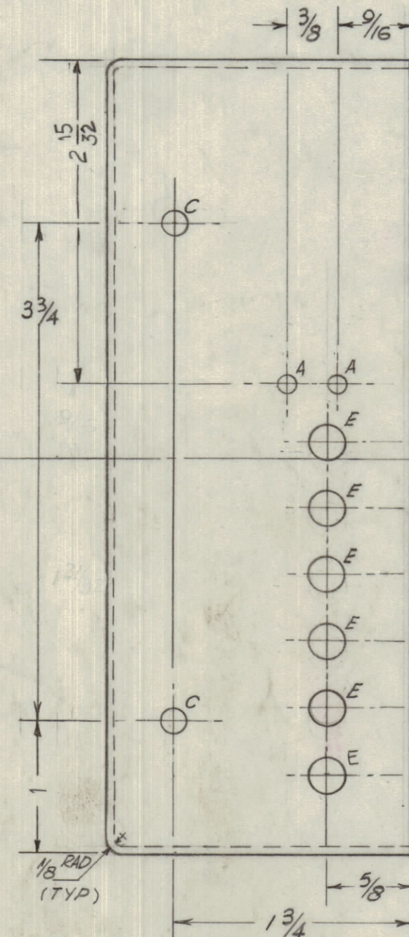
DETAIL J FOR #8-32 FHS.
