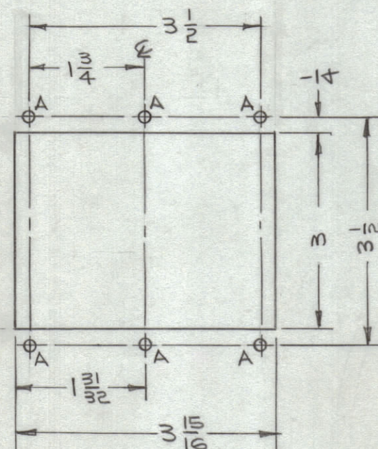
DETAIL B CUTOUT 1 REQD
