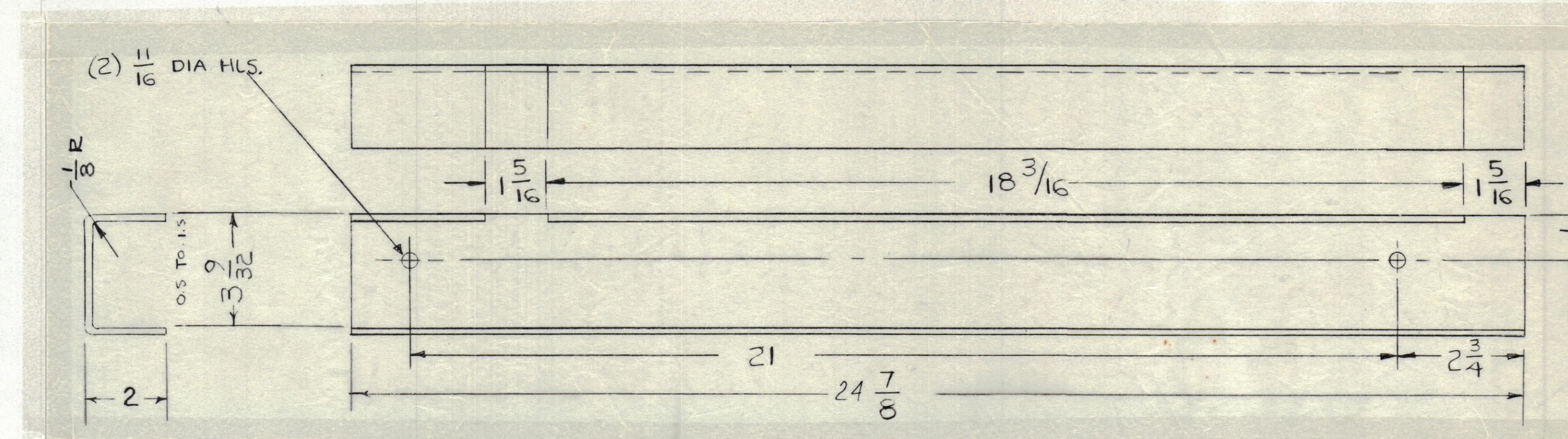
DETAIL "B" BASE CHANNEL 2-REQ. *10 GA. GALVANIZED STEEL
