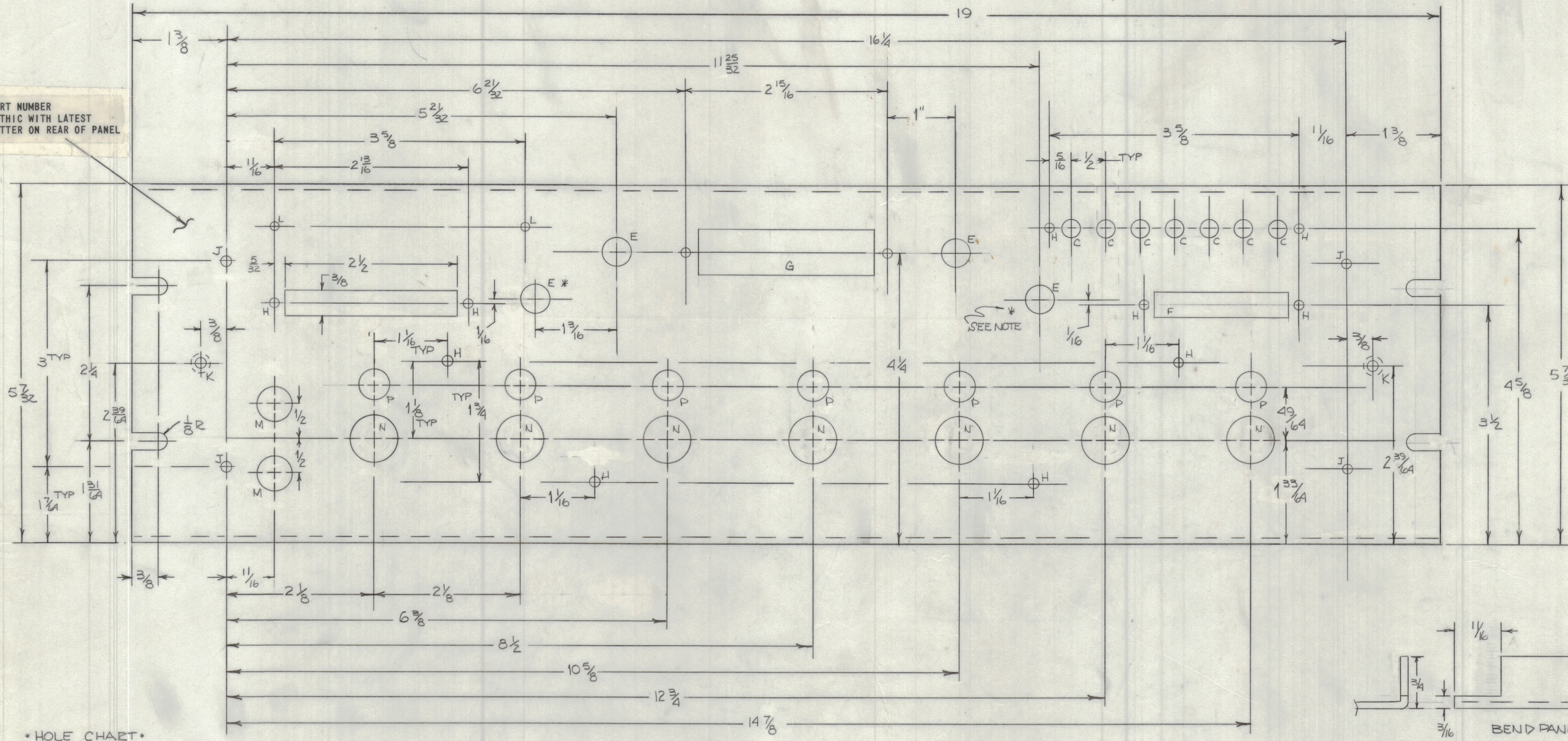
* HOLE CHART *
