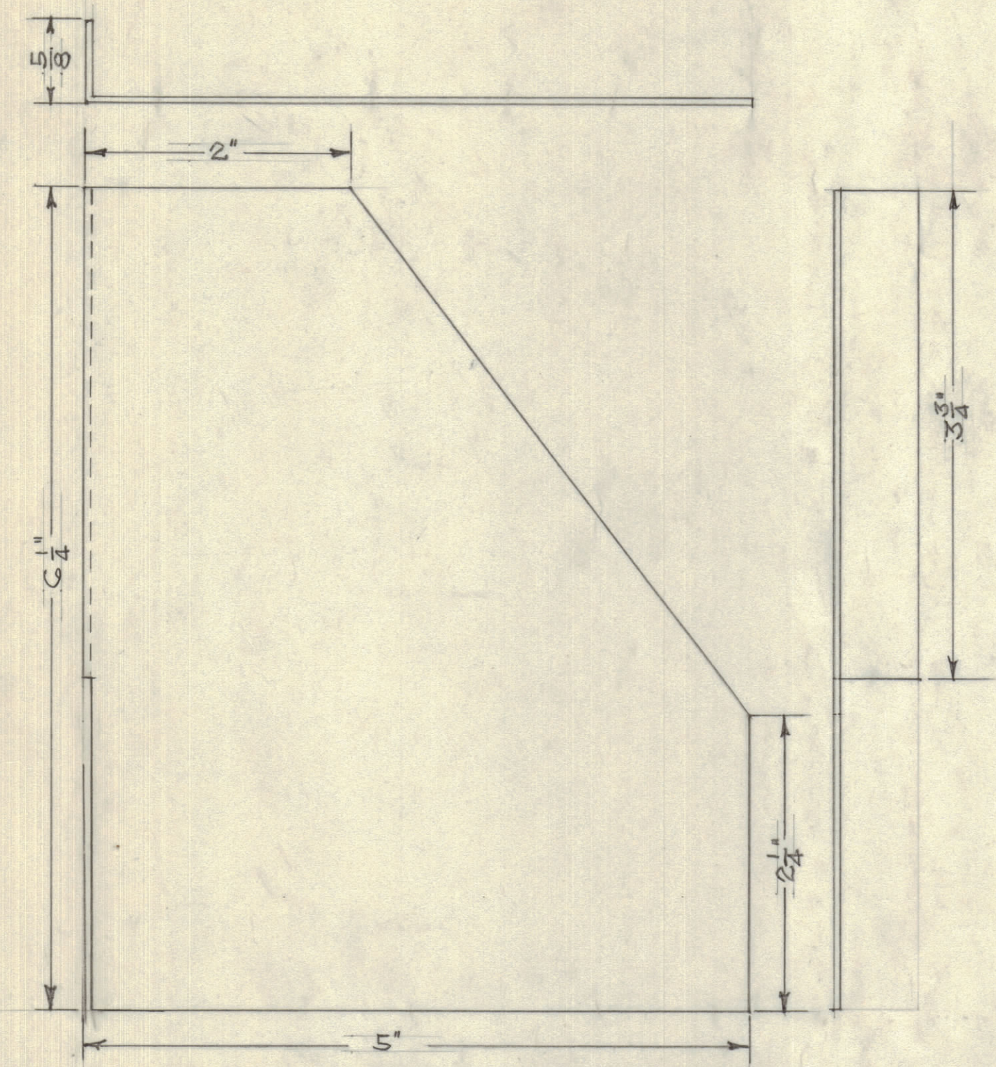
LEFT SUPPORT BRACKET
