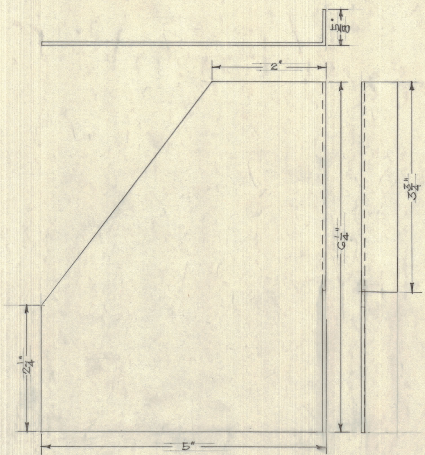
RIGHT SUPPORT BRACKET
