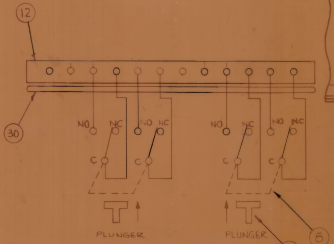
TYPICAL WIRING DIAGRAM
