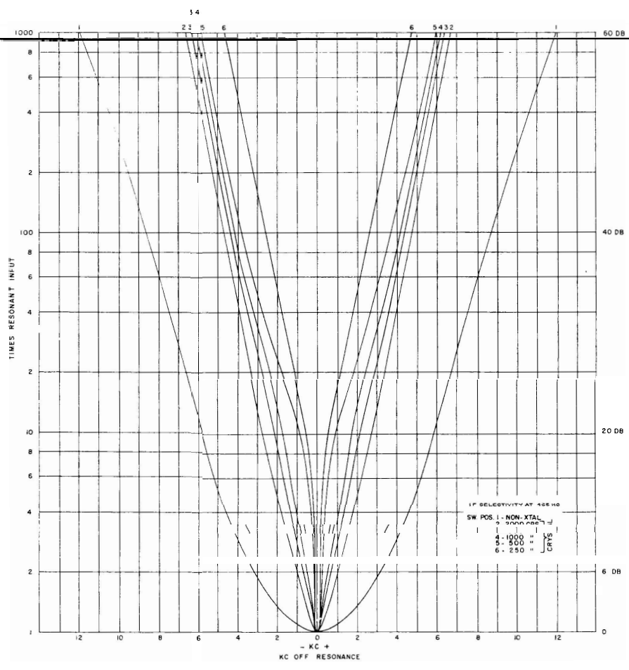
Figure 5-2. IF Selectivity Curves
