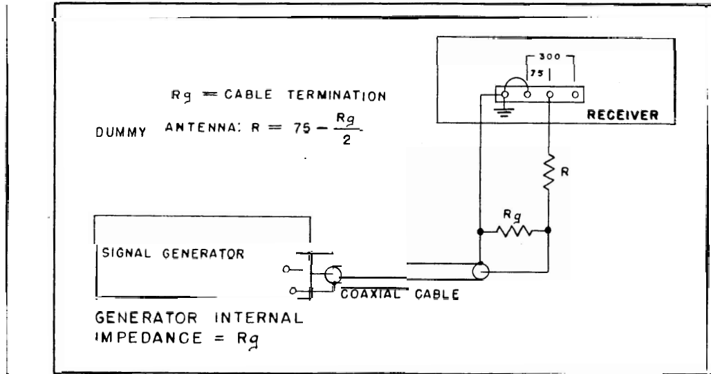
Figure 4-3. Signal Generator Connections for RF Alignment
