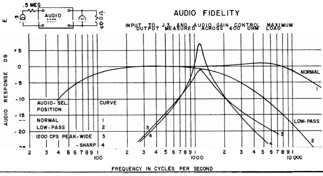
Figure 5-1. Audio Fidelity Curves
