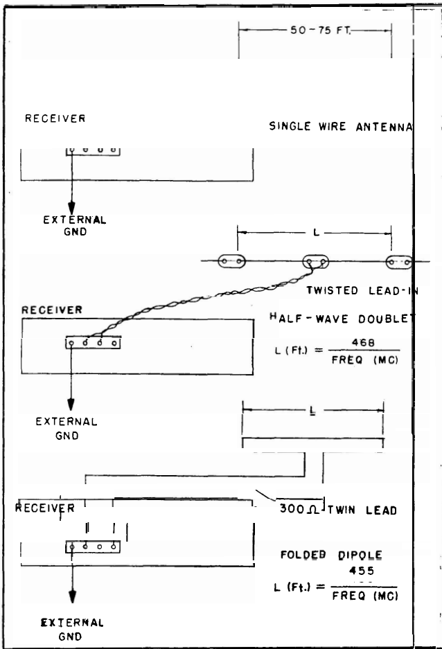
Figure 2-1. Typical Antenna Installation
