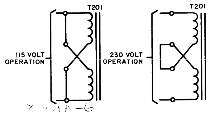
Figure 2-1. Installation Diagram Showing 115- vs 230-Volt Power Supply Connections
