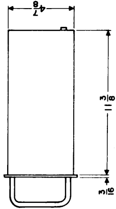
DA-101-70/U DISTRIBUTIVE AMPLIFIER
