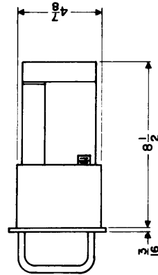
PS-7 POWER SUPPLY
