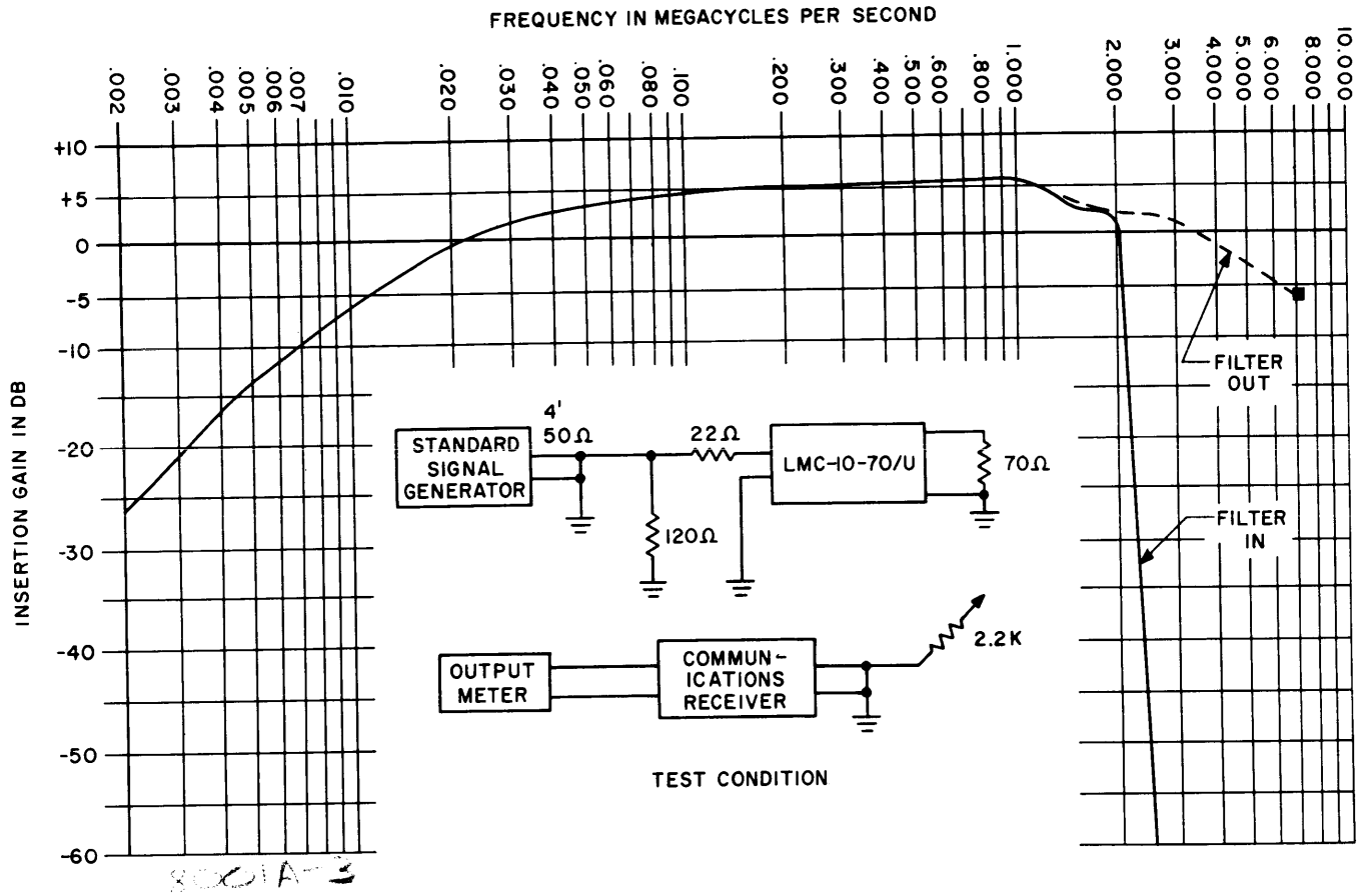
Figure 1-2. Typical Insertion Gain Characteristics, LMC-10-70/U
