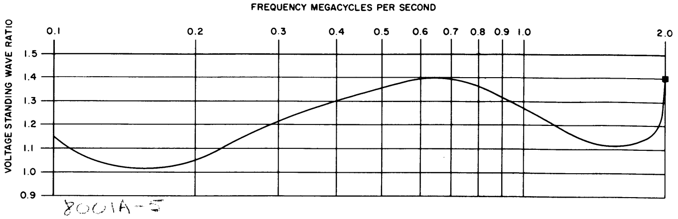
Figure 1-4. Typical Input Impedance Characteristics, LMC-10-70/U (Filter In)
