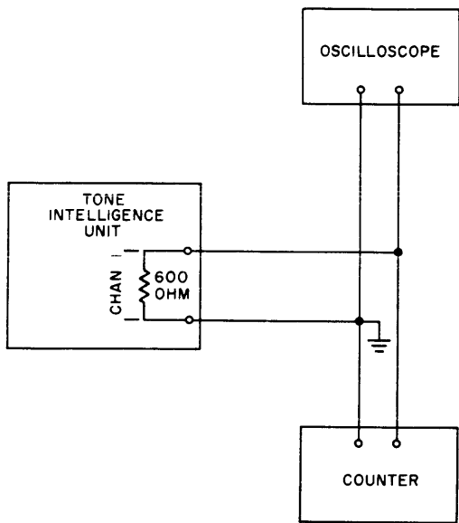
Figure 6-1. Test Setup No. 1
