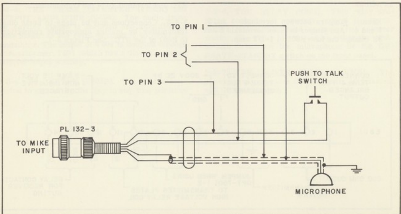
Figure 3-3. Microphone Connections
