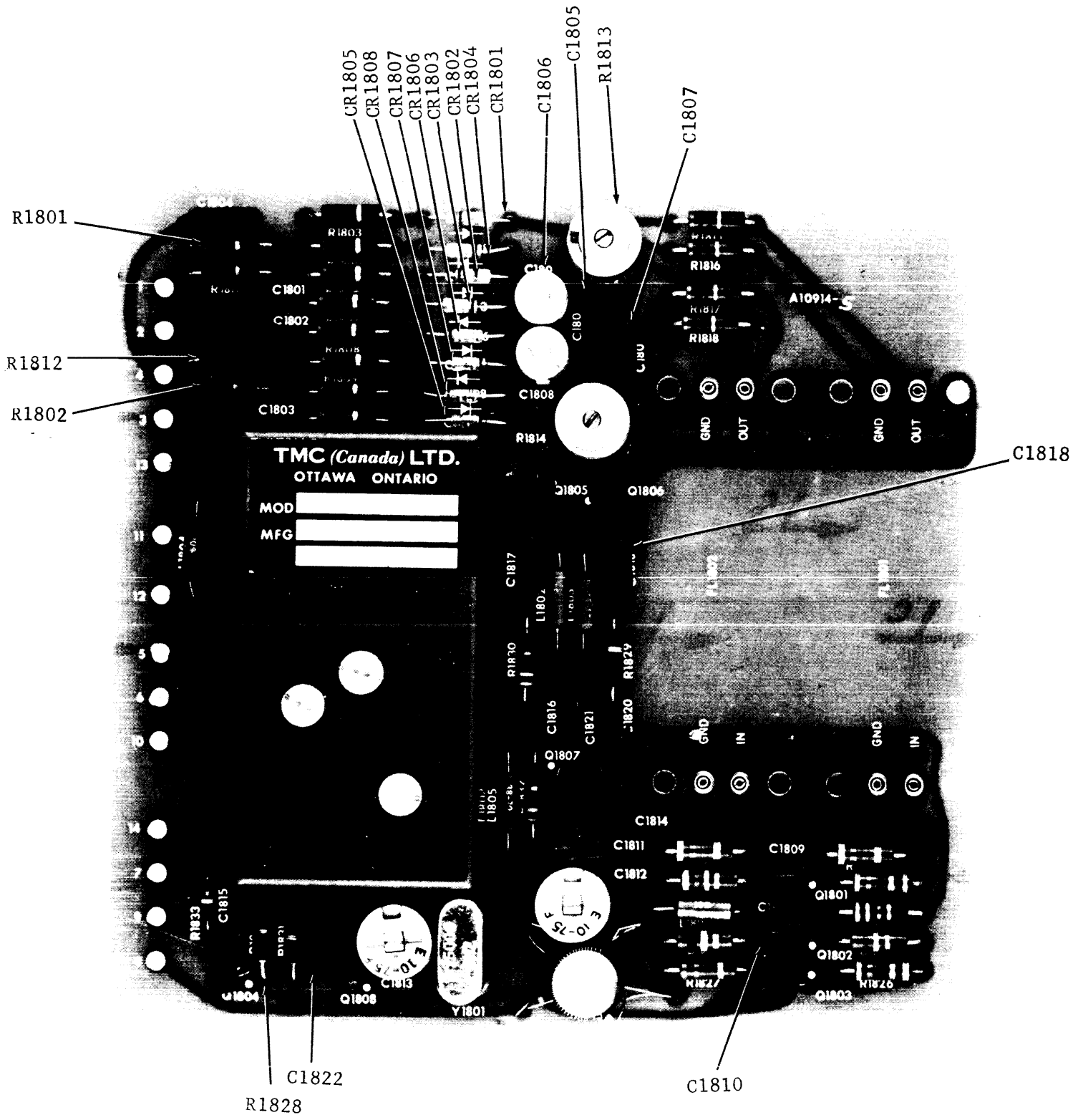
Figure 5-4 XMIT IF board A9 parts location
