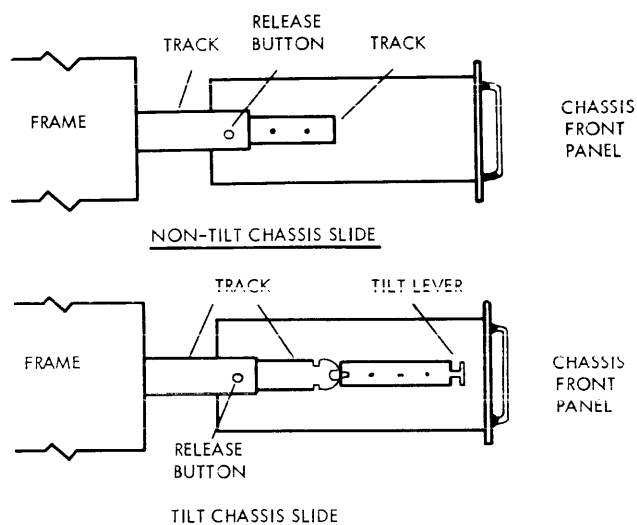
Figure 2-1. Tilt-Lock Slide Mechanism
