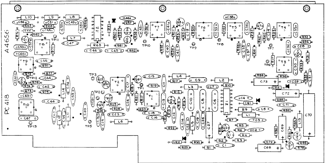
Figure 5-8. Carrier Generator Z101, Component Location
