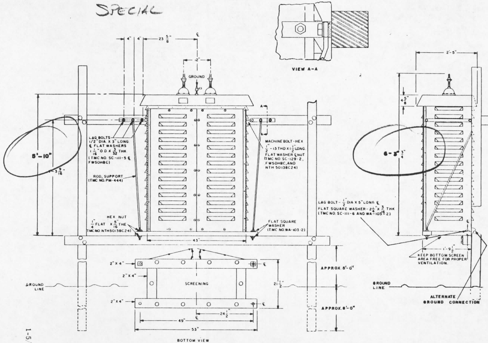
Figure 3. Installation Diagram
